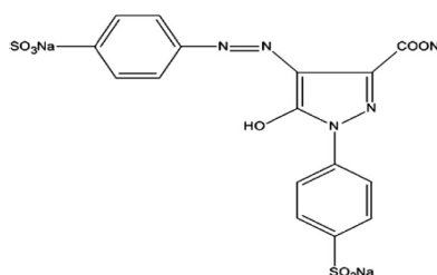
Fig. 1. Structure of tartrazine dye
