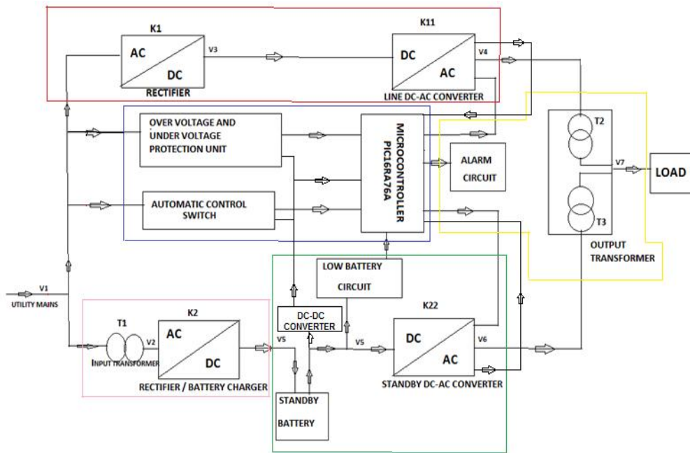
Fig. 1. Block diagram of the UPSz
