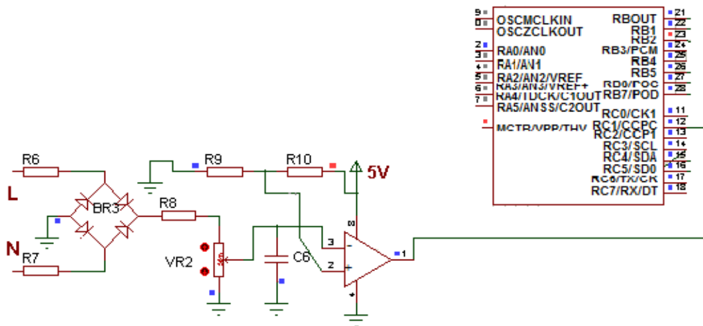
Fig. 11. Diagram of over voltage protection circuit
