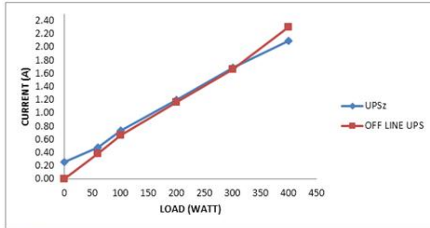
Fig 25 A graph of load against current for both the UPSz and the offline UPS at 180V AC input voltage.
