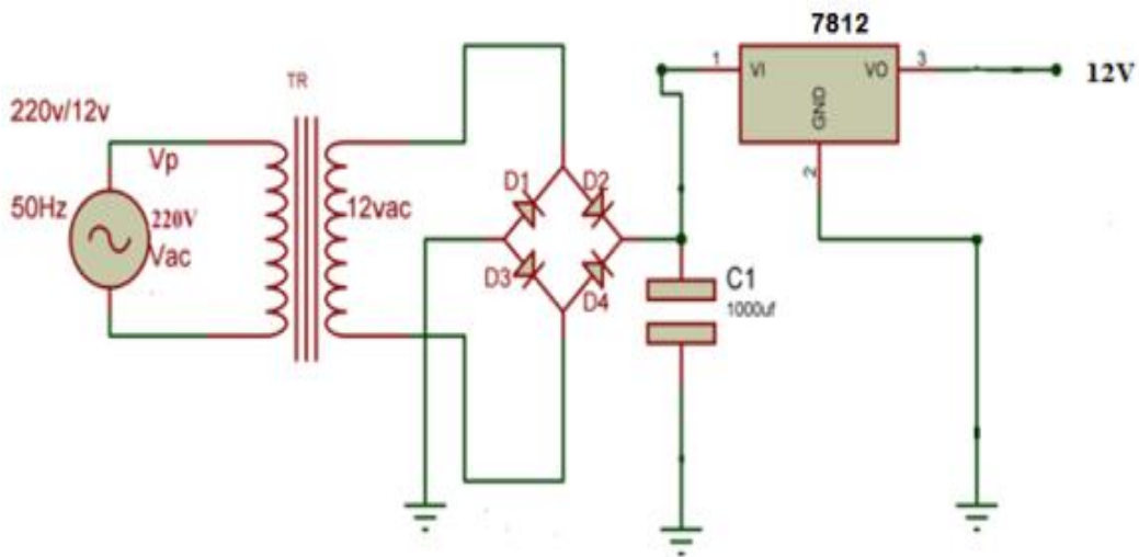
Fig. 5. Circuit diagram of the rectifier K2 with transformer T_1
