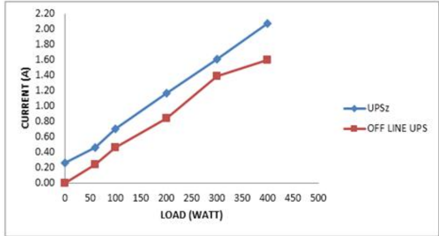
Fig 22 A graph of load against current for both the UPSz and the offline UPS at 240V AC input voltage.
