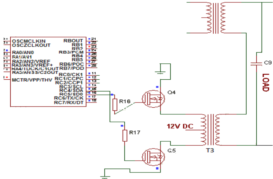
Fig. 7. Circuit diagram of the standby DC-AC converter interfacing the transformer T 3
