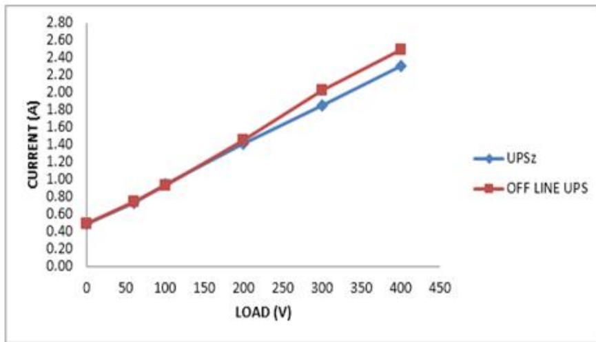
Fig 28 A graph of load against current for both the UPSz and the offline UPS during mode II
