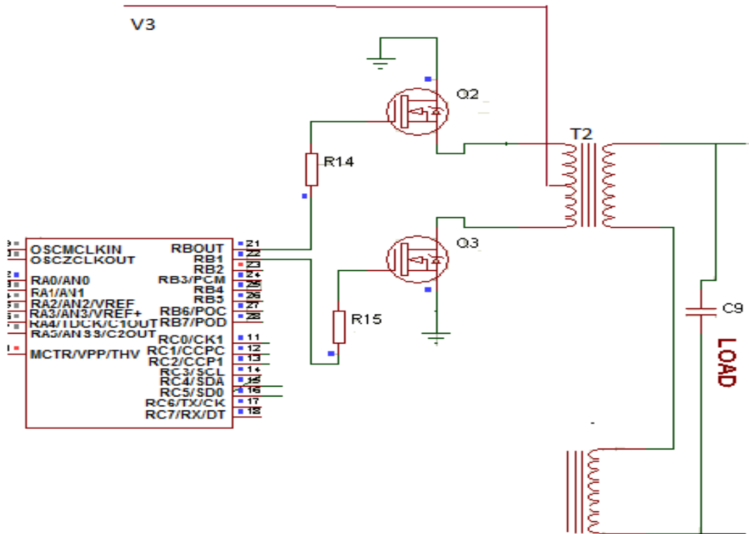
Fig. 4. Half-bridge DC-AC converter connected to a microcontroller
