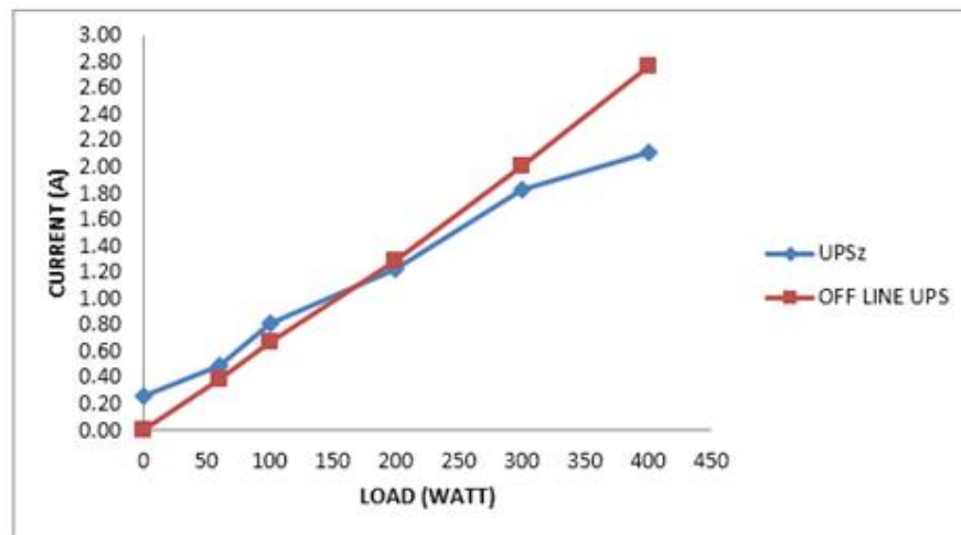
Fig 26 A graph of load against current for both the UPSz and the offline UPS at 160V AC input voltage
