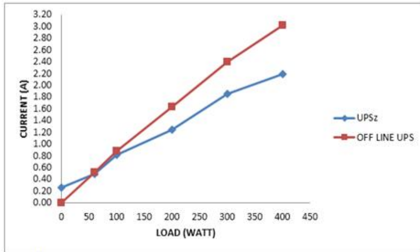
Fig 27 A graph of load against current for both the UPSz and the offline UPS at 140V AC input voltage.
