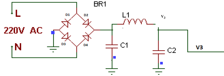
Fig. 3. Circuit diagram of the rectifier (k1) with filters
