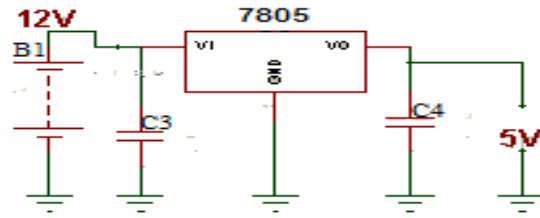
Fig. 6. Diagram of the DC-DC converter connected to the battery (B1)
