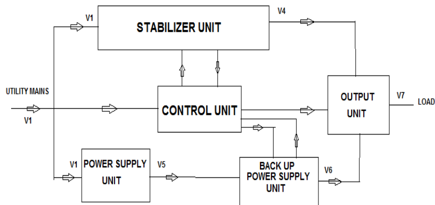
Fig. 2. Simplified block diagram
