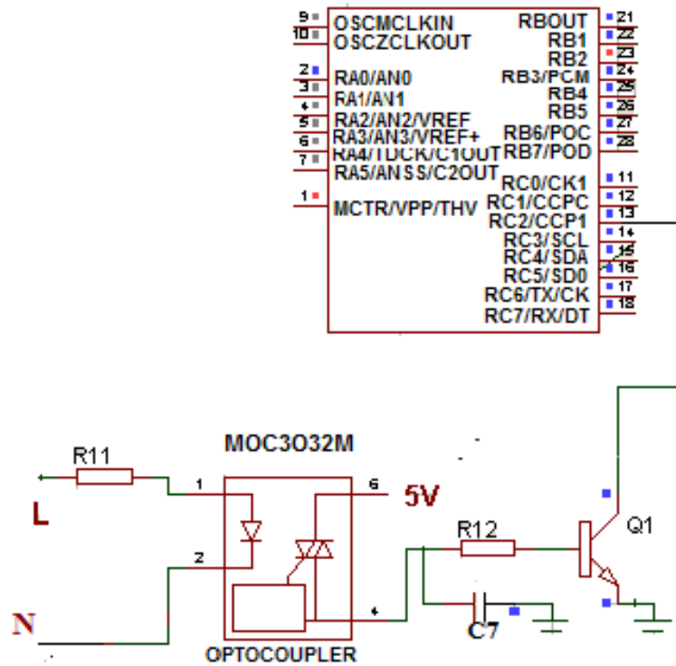
Fig. 10. Circuit diagram of the automatic control switch interfacing the microcontroller
