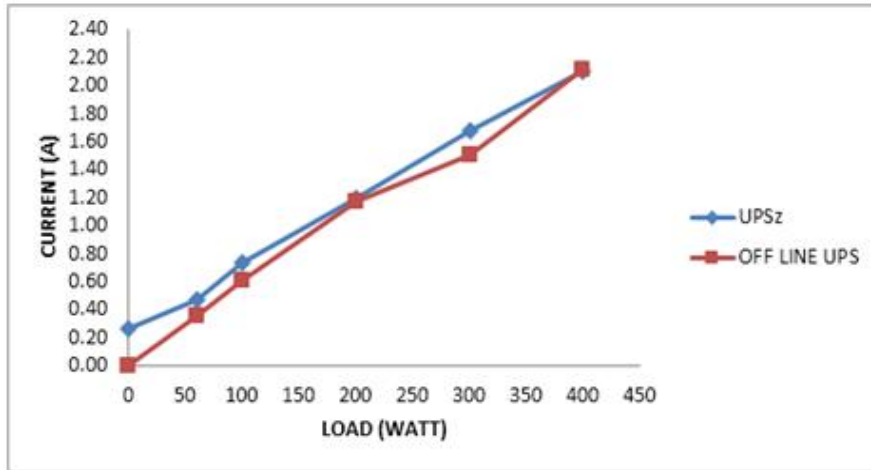
Fig 24 A graph of load against current for both the UPSz and the offline UPS at 200V AC input voltage.
