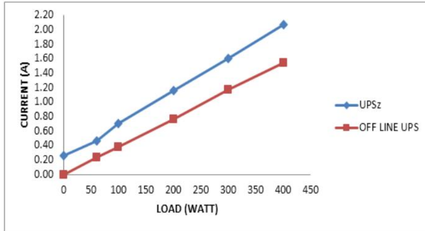
Fig21: A graph of load against current for both the UPSz and the offline UPS at 260V AC input voltage.
