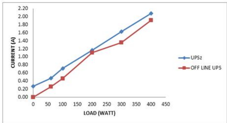
Fig 23 A graph of load against current for both the UPSz and the offline UPS at 220V AC input voltage.
