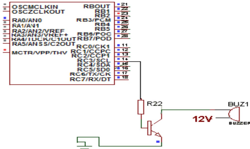
Fig. 14. Diagram of the UPSz alarm unit
