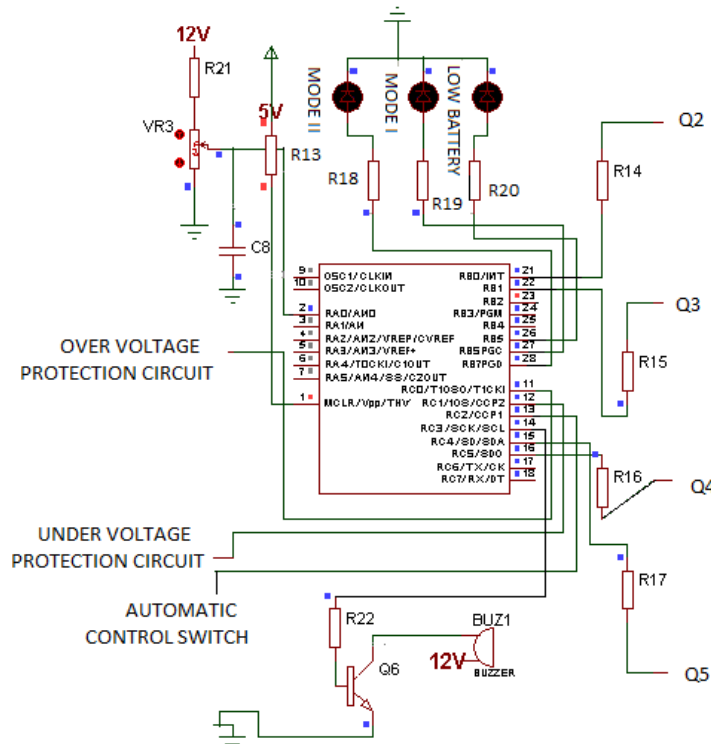
Fig. 9. The microcontroller interfacing various sections of the UPSz
