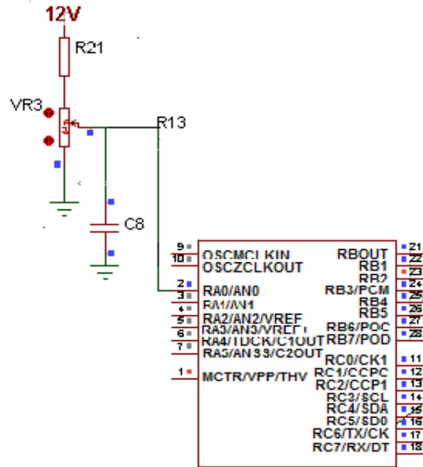
Fig. 8. The low battery circuit interfacing with the microcontroller
