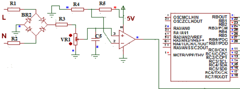
Fig. 12. Diagram of over voltage protection circuit
