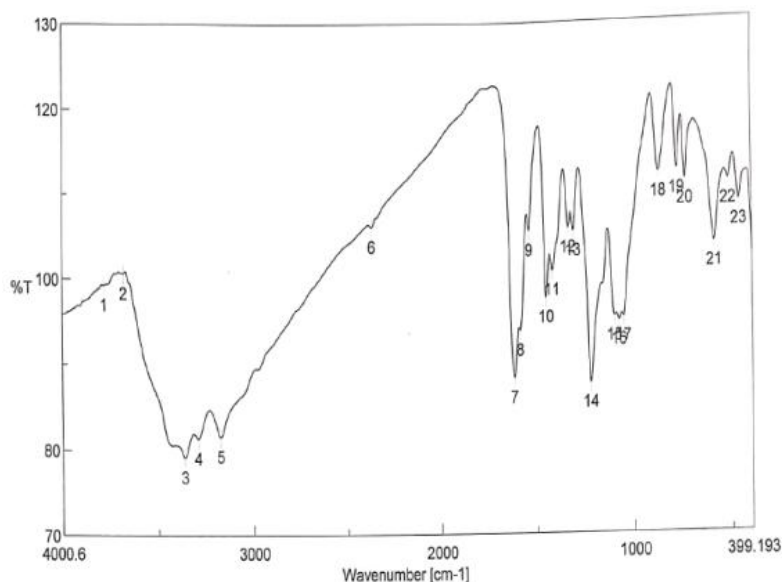
IR spectroscopy of compound 3a
