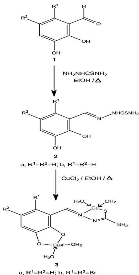
Scheme 1. Synthesis of the compounds (2a, 2b, 3a & 3b)
