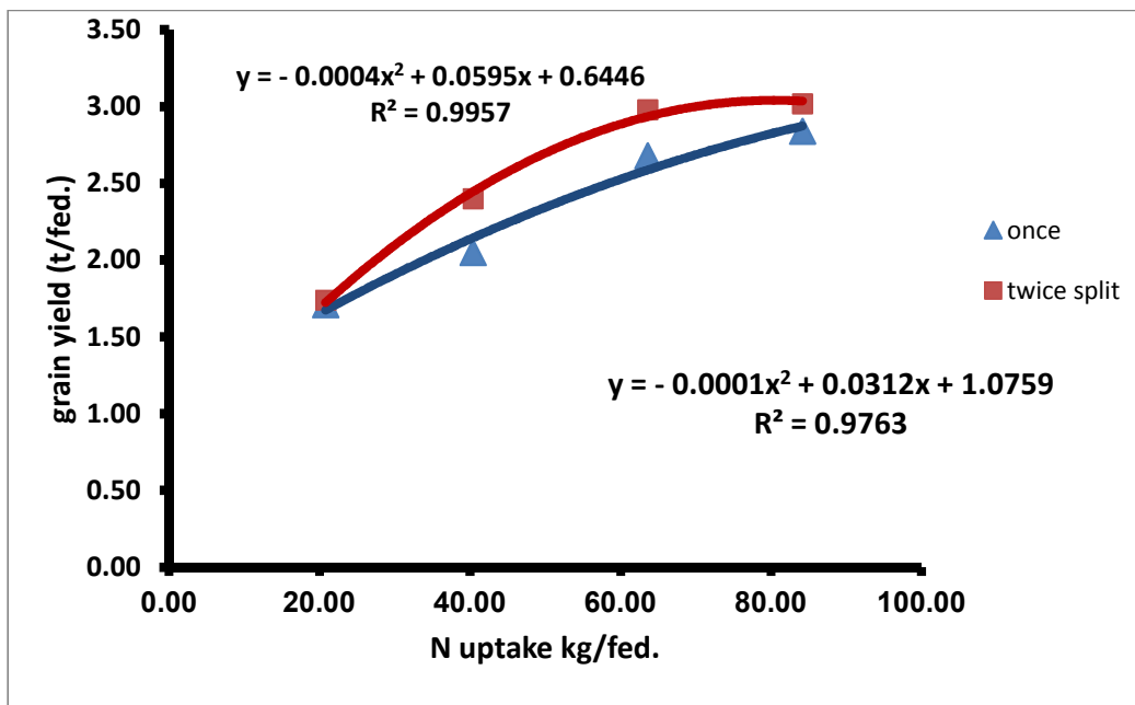
Fig. 1. Relationship between total N uptake and wheat grain yields
