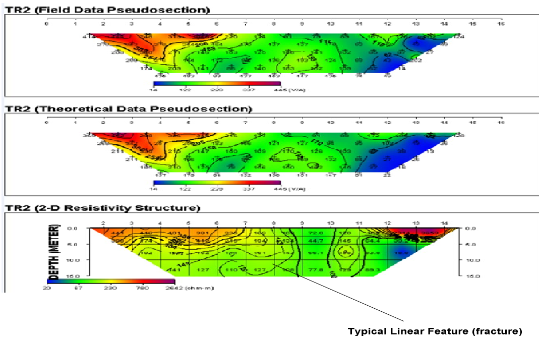
Fig. 6b. Dipole - Dipole Horizontal Profiling along traverses 2
