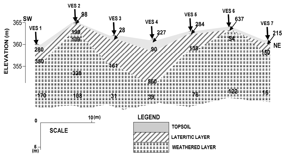
Fig. 5a. Geoelectric SECTION along traverse one
