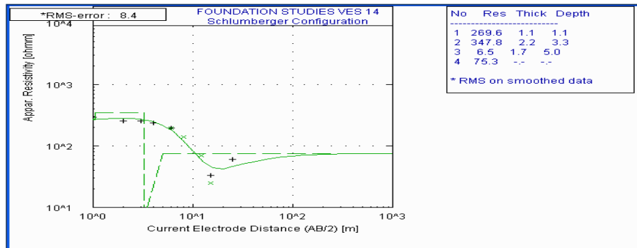
Fig. 4C. Typical 'KH' sounding curve
