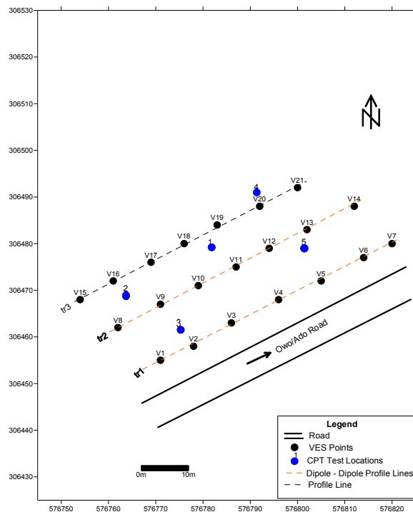
Fig. 3. Data acquisition map of the study area
