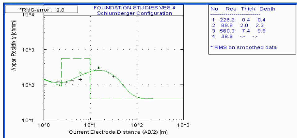
Fig. 4b. Typical 'HK' sounding curve
