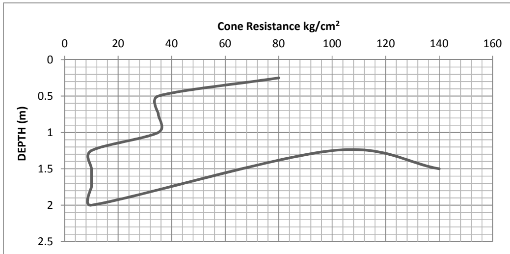
Fig. 7d. CPT Test carried out in point 4
