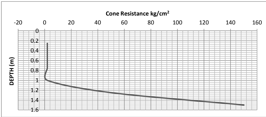
Fig. 7a. CPT Test carried out in point 1
