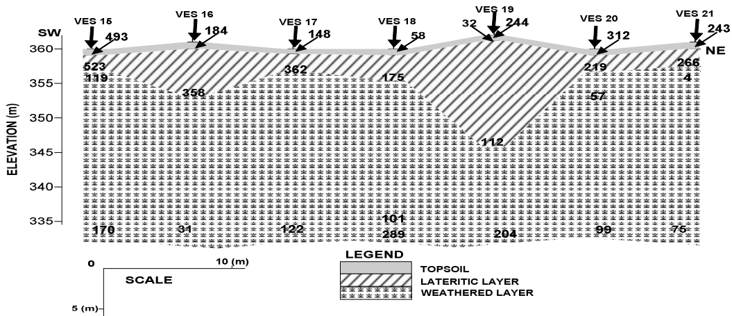
Fig. 5c. Goelectric section along traverse three
