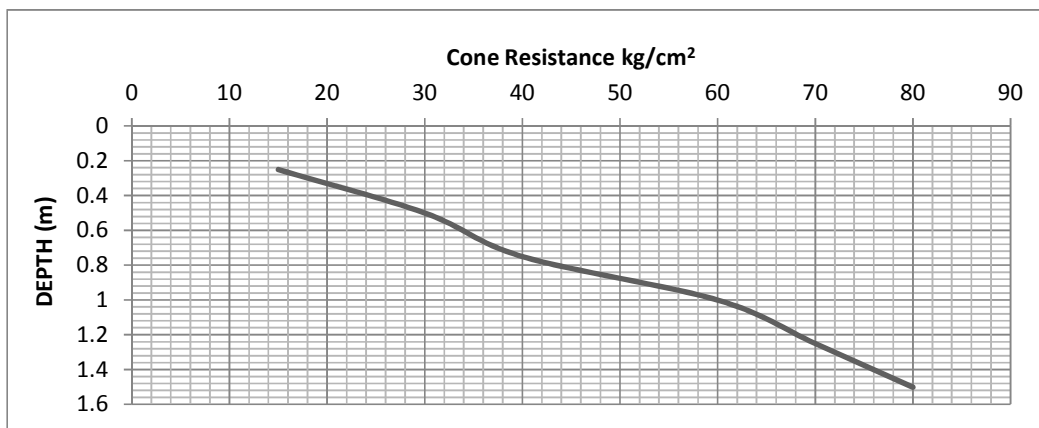
Fig. 7e. CPT Test carried out in point 5
