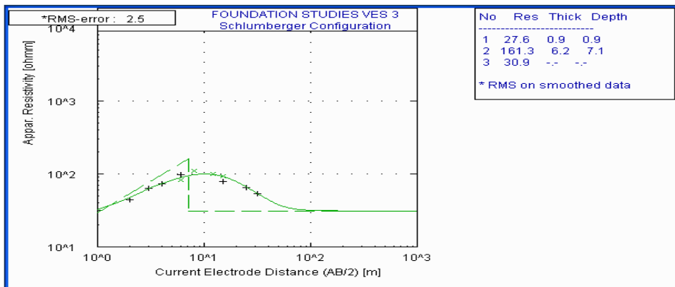
Fig. 4a. Typical 'K' sounding curve
