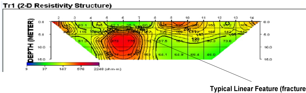
Fig. 6a. Dipole-Dipole Horizontal Profiling along traverses 1
