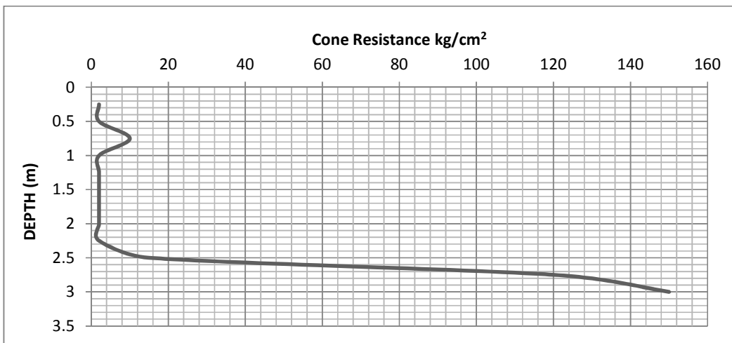
Fig. 7b. CPT Test carried out in point 2
