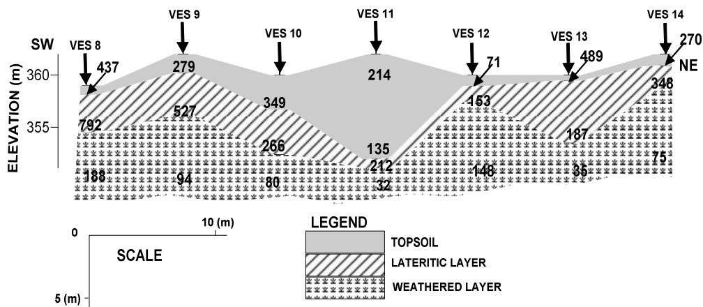
Fig. 5b. Geoelectric Section along Traverse two
