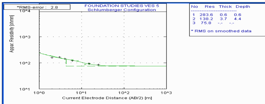
Fig. 4d. Typical 'Q' sounding curve
