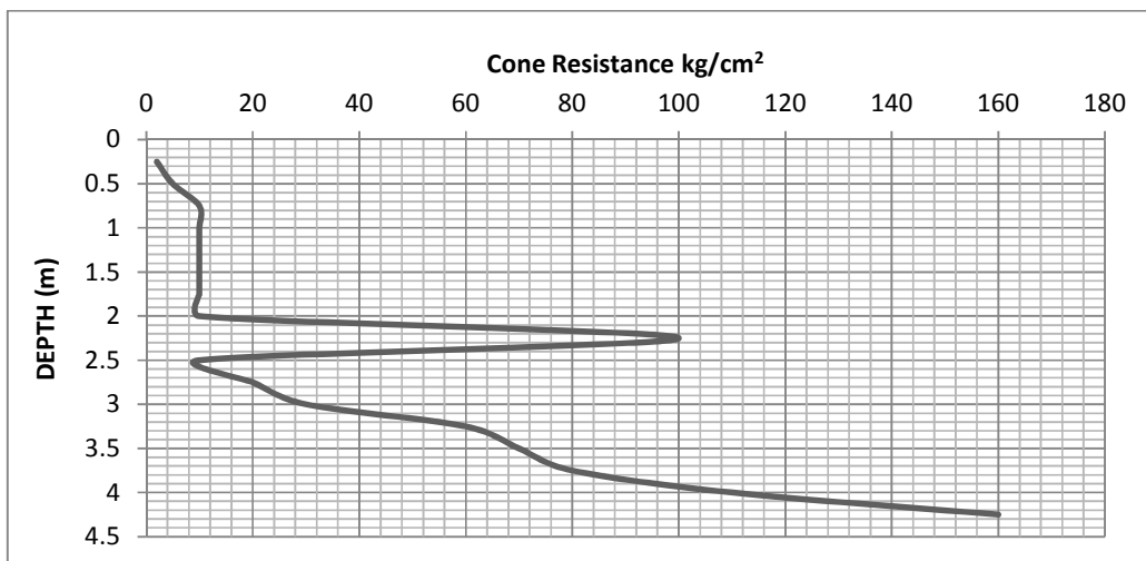
Fig. 7c. CPT Test carried out in point 3
