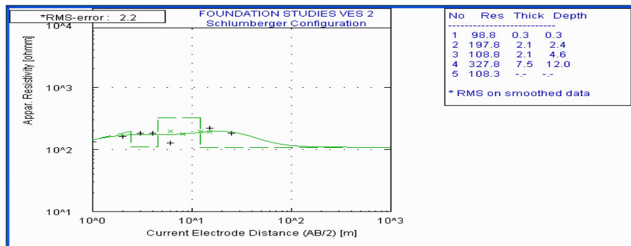
Fig. 4e. Typical 'KHK' sounding curve
